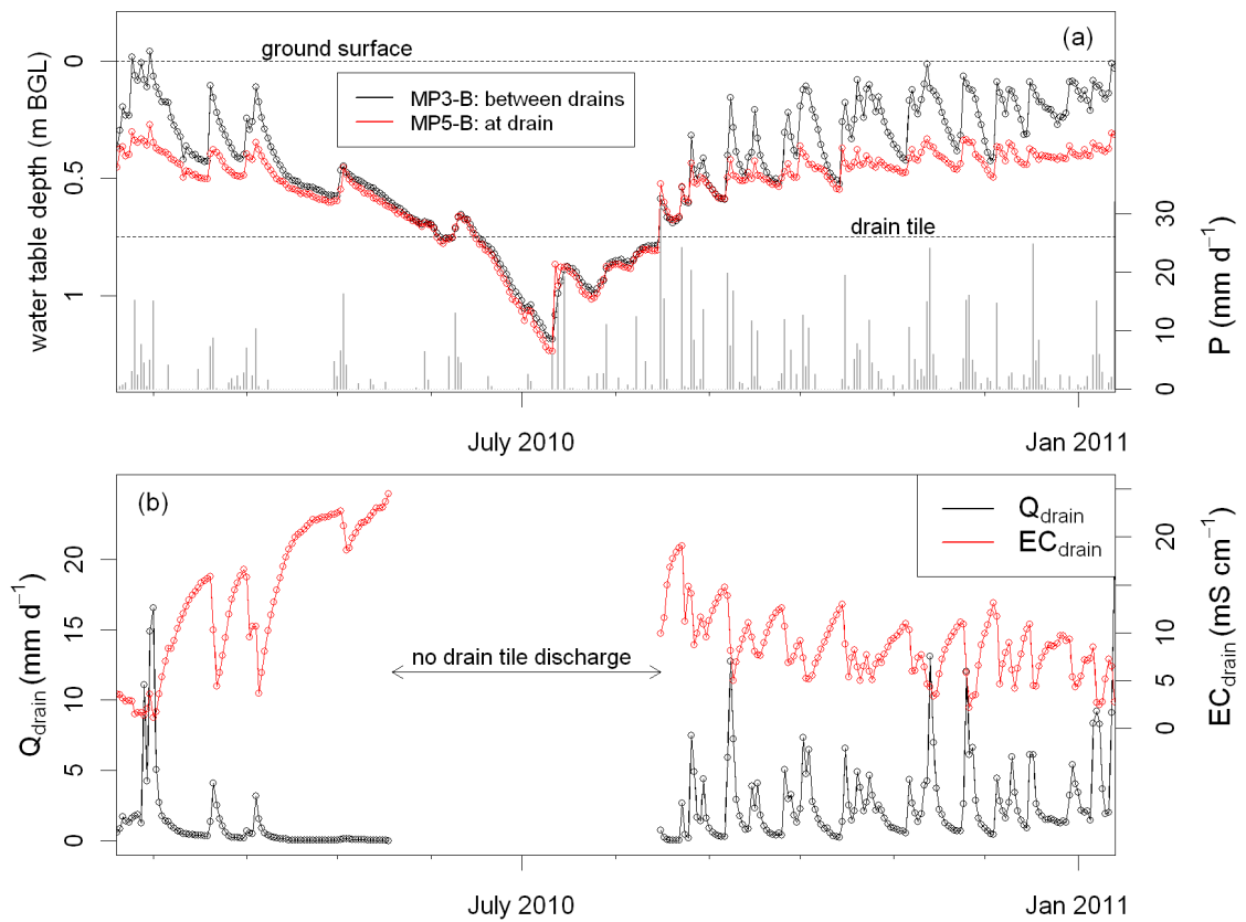
Fig. H2. Graph showing times series at site B (site B is Drains2Buffer-pilot area in Kerkwerve) of (a) the water table at a drain tile and between two drain tiles, and (b) Q_{\text{drain}} and EC_{\text{drain}} . Water table elevations above the ground surface indicate conditions of surface ponding.
