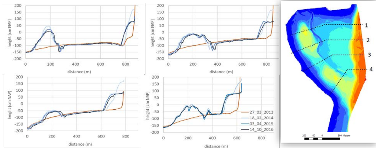
Figure 5-3. Cross-section 1, 2, 3 and 4.
