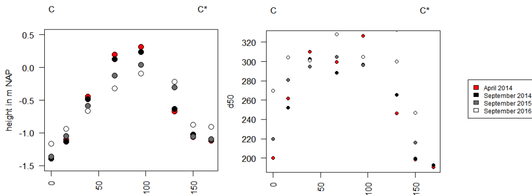
Figure 6-3. Change in elevation (left) and median grain size (right) along transect C-C* on the main sand nourishment. See Fout! Verwijzingsbron niet gevonden. for the position of the transects.
