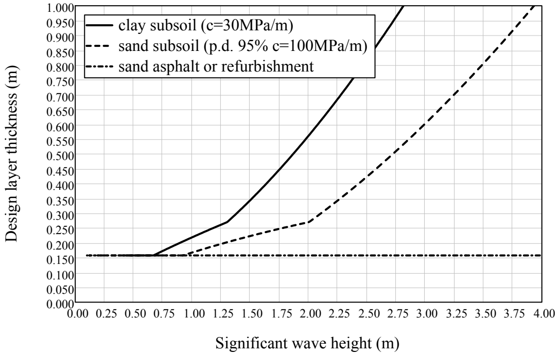
Limestone 30/60 mm ( E=3000\text{MPa} , \sigma_{\text{max}}=0.5\text{MPa} )
